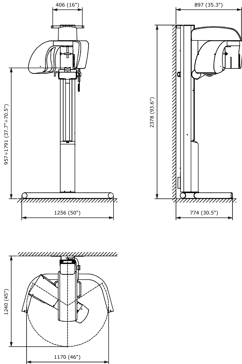
Figure 4-1: I-MAX EASY overall dimension
